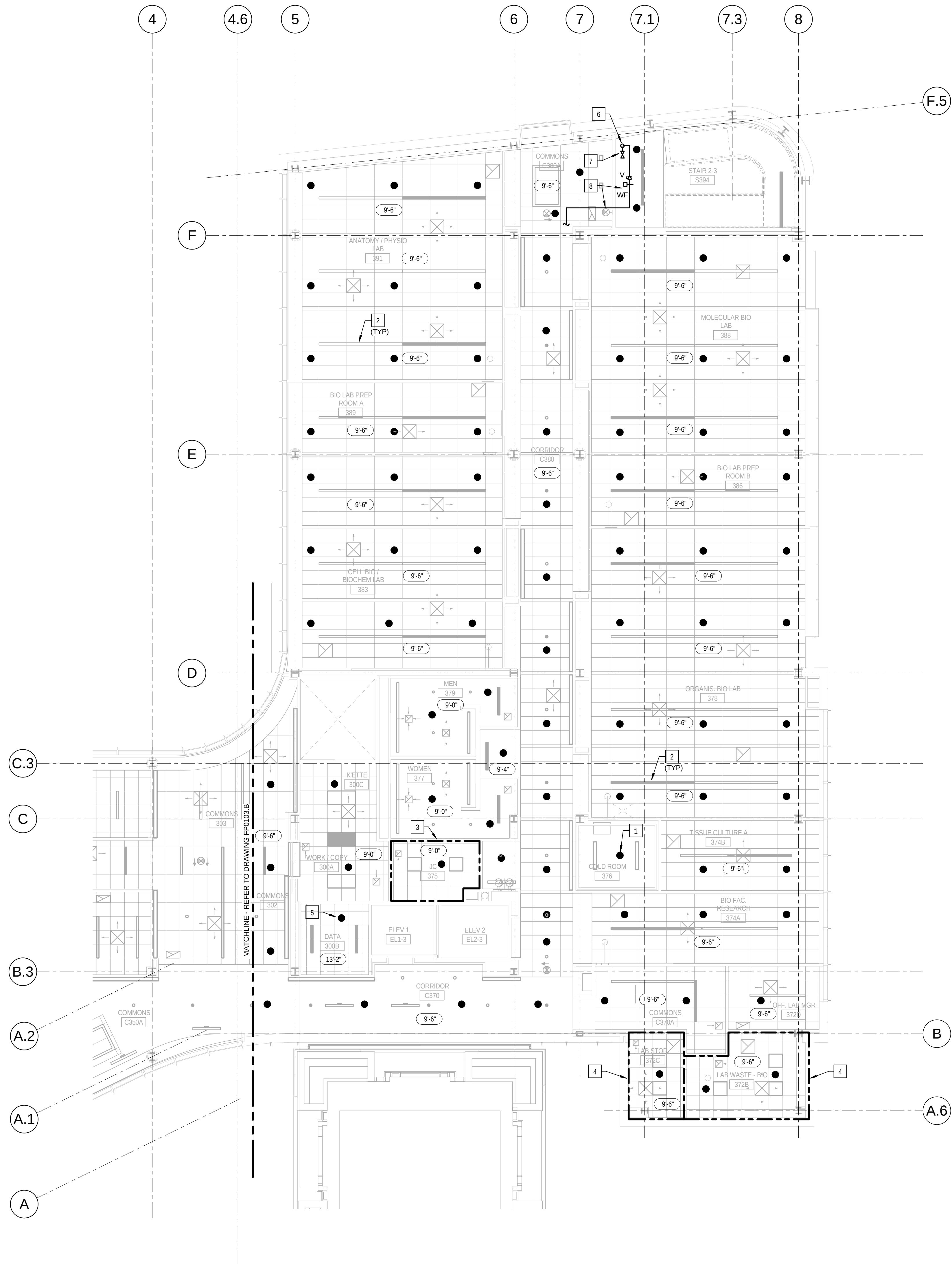
1 LEVEL 03 AREA A FLOOR PLAN - FIRE PROTECTION 1/8" = 1'-0"
